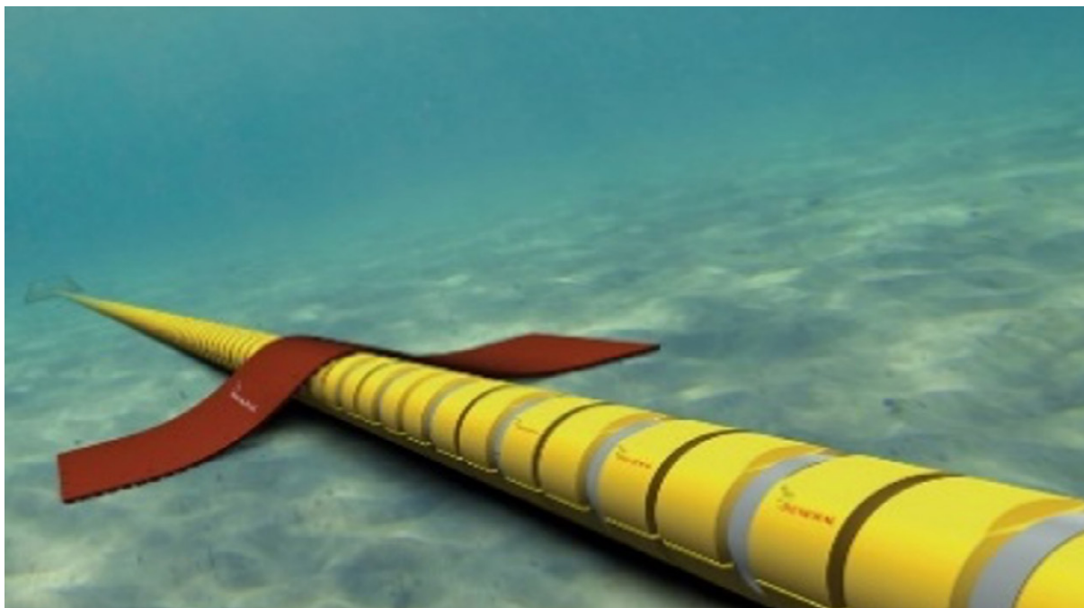
Figure 14: Abrasion Protection (Courtesy: Balmoral Offshore) 15
