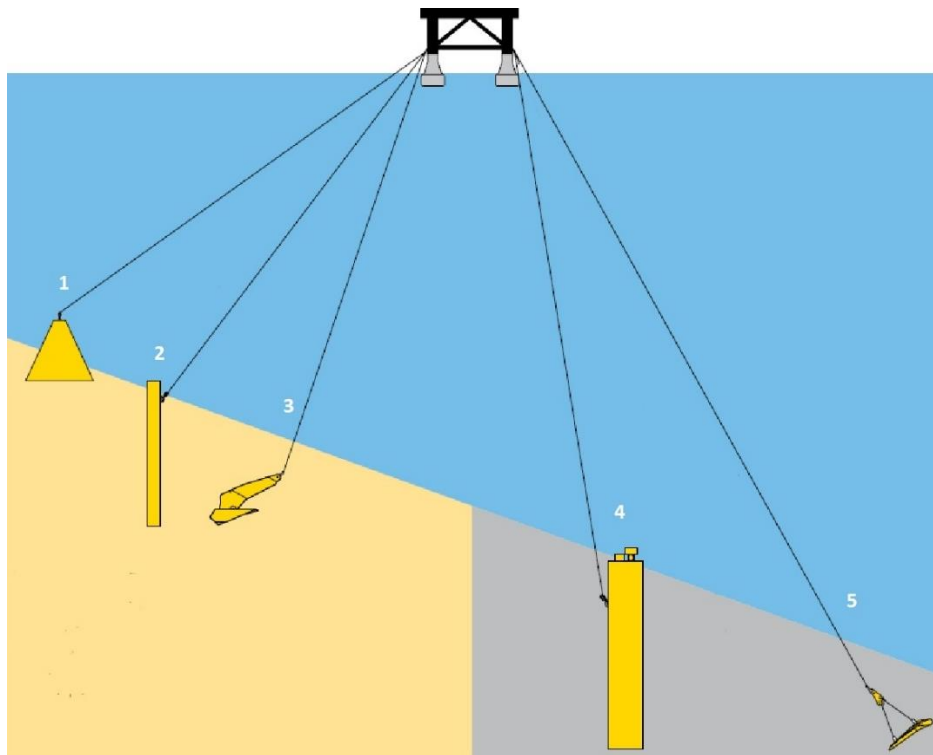
Figure 9: Visual Representation of Anchor Types [16]
