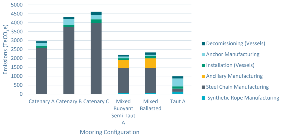
Figure 28: Base Case Mooring Configuration Carbon Emissions
