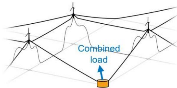
Figure 19: Shared Anchor Concept Geometries [26]
