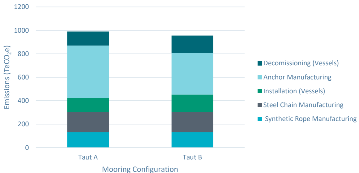
Figure 32: Alternative Taut Configuration Carbon Emissions Comparison
