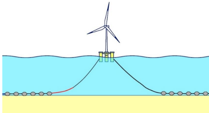
Figure 22: Typical Ballasted Catenary System [6]
