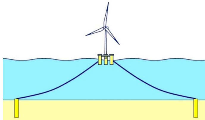
Figure 24: Typical Taut Mooring System [6]
