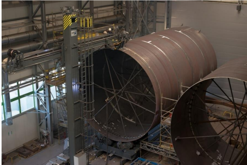
Figure 13: Suction Bucket Production with Semi Automated Weld Plant [19]
