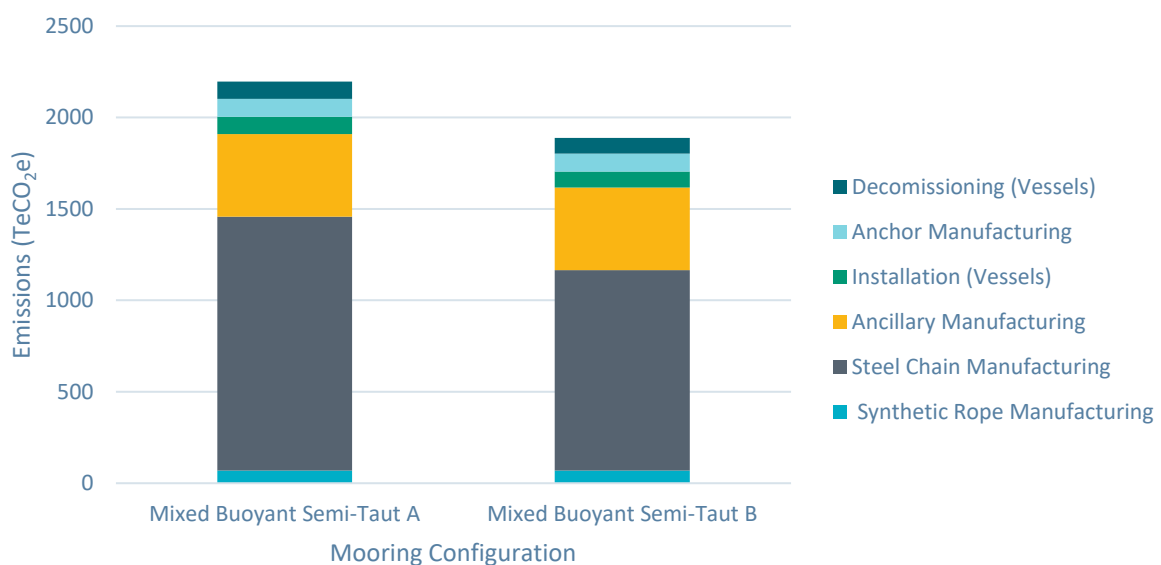
Figure 31: Alternative Mixed Buoyant Semi-Taut Carbon Emissions Comparison
