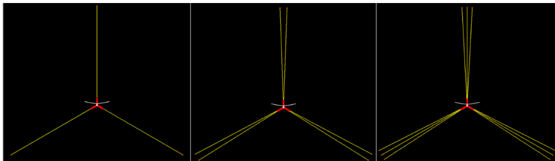
Figure 21: Example Layout of FOWT Mooring Configuration (Left: 3-Line, Middle: 3 by 2, Right: 3 by 3)
