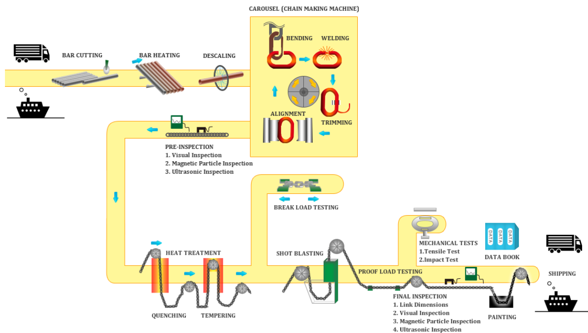
Figure 4 : Steel Chain Manufacturing Process Diagram (Adapted) [11]
