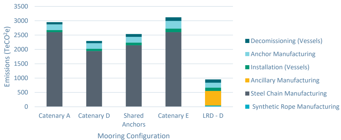
Figure 29: Alternative Catenary Mooring Configuration Carbon Emissions Comparison
