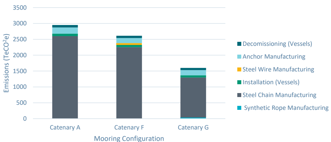
Figure 30: Hybrid Catenary Carbon Emissions Comparisons
