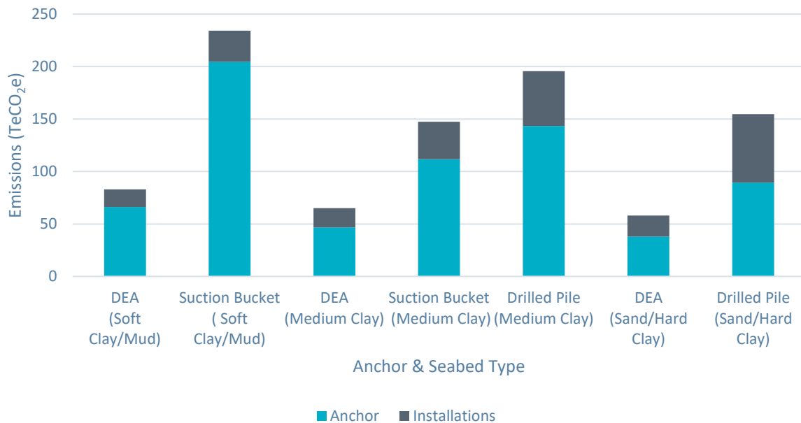
Figure 26: Emissions considering Anchor Types and Seabed Conditions (12,000kN UHC)
