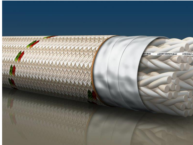
Figure 7 : Synthetic Rope Construction [14]
