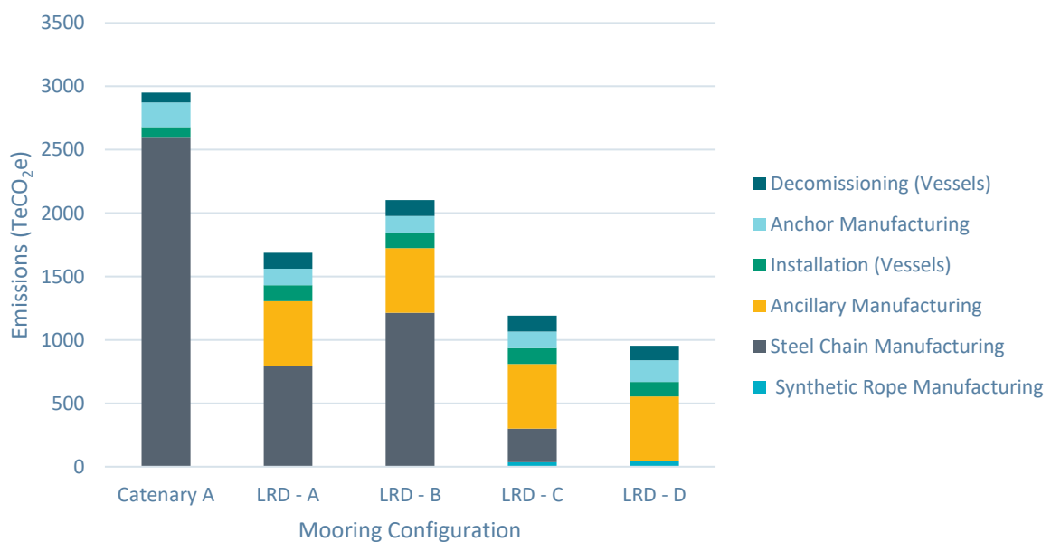
Figure 33: Alternative Catenary Configuration with LRD Optimisation Carbon Emissions Comparison
